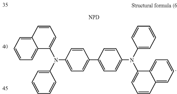
Structural formula (2)
