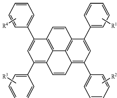
Structural formula (1)
