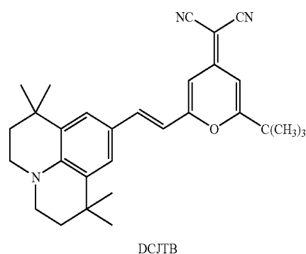
Structural formula (9)
