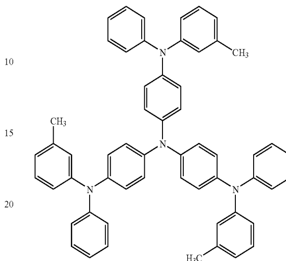
5 Structural formula (4)
