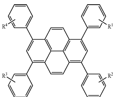
Structural formula (1)
