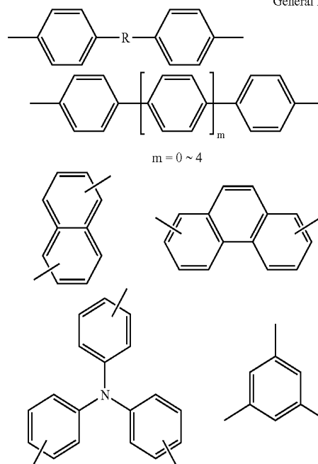
General formula (1)
