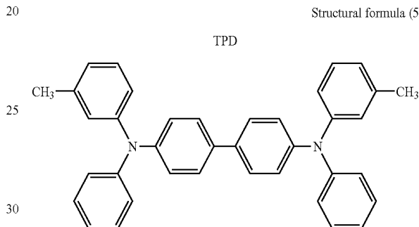
Structural formula (5)
